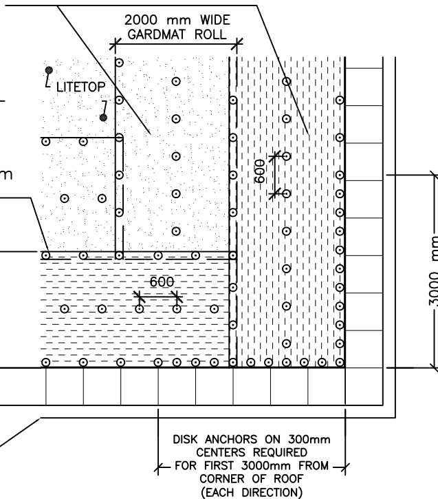
LAYOUT AND ANCHORING
